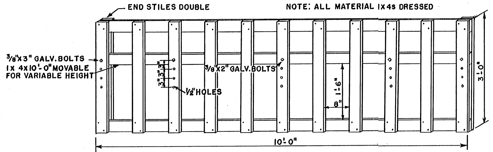
PANEL FOR CREEP FEEDING
