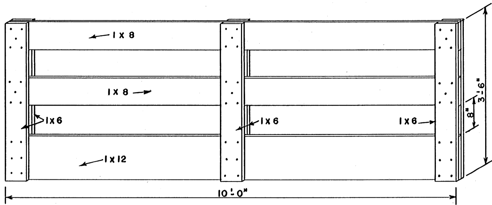
PANEL FOR LAMBS NOTE: MAY BE USED FOR FENCING A LOT AND AS A FEED RACK
