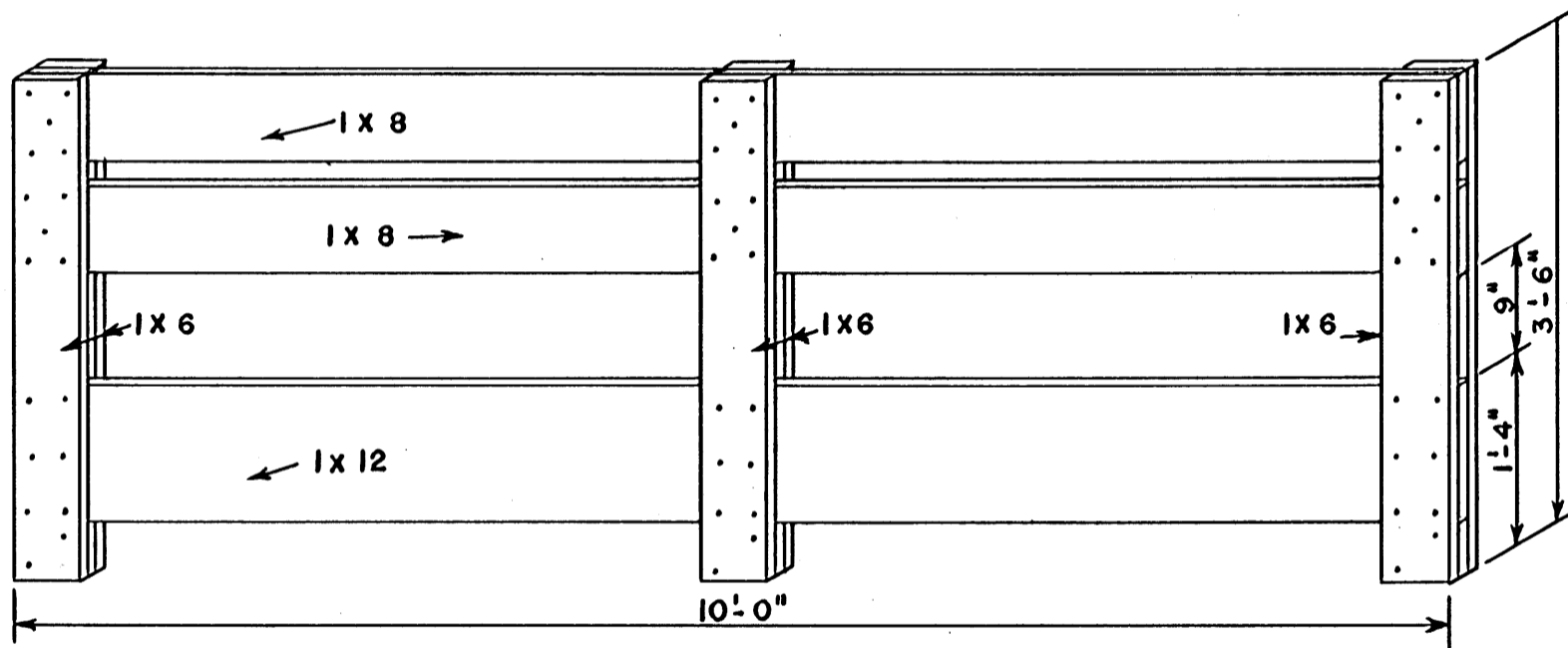
PANEL FOR EWES
