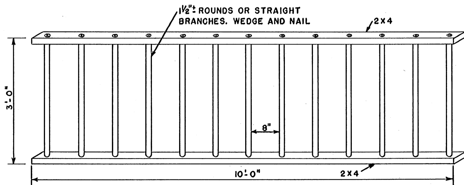
CREEP PANEL
