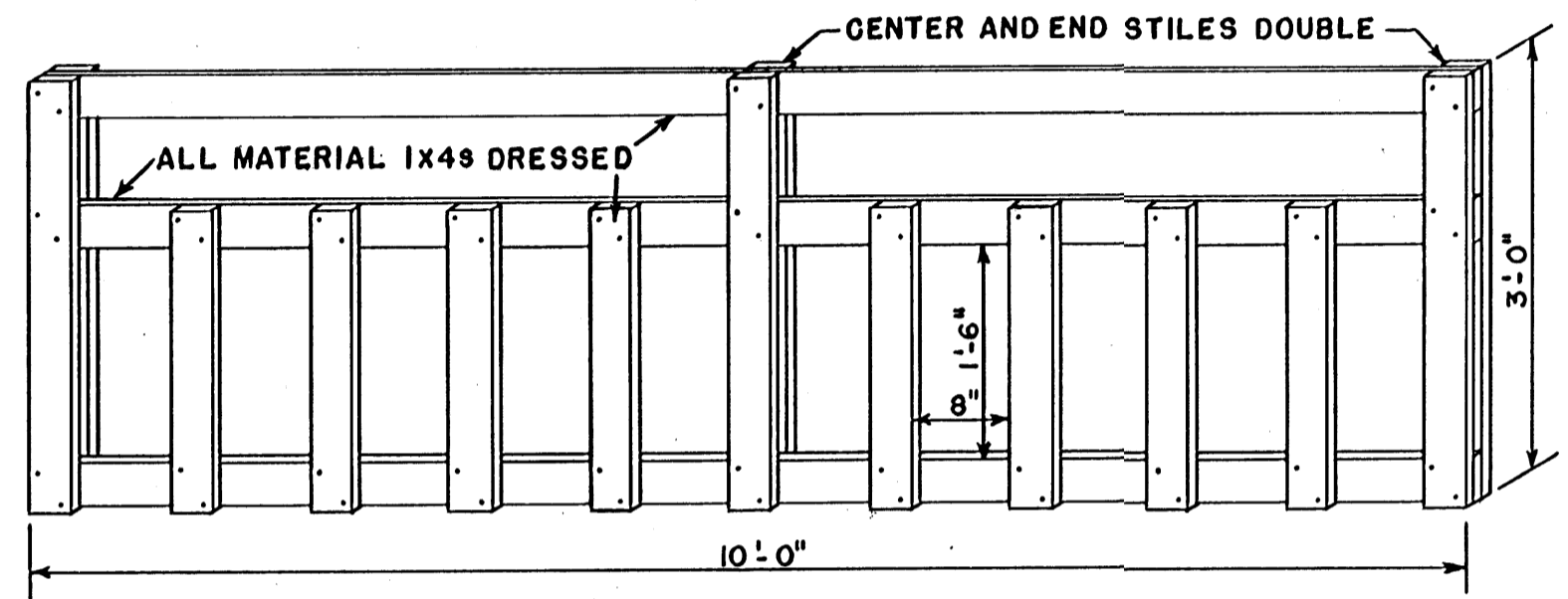
PANEL FOR CREEP FEEDING
